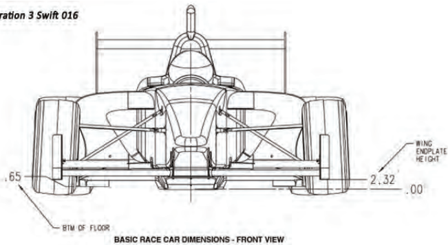
BASIC RACE CAR DIMENSIONS - FRONT VIEW
